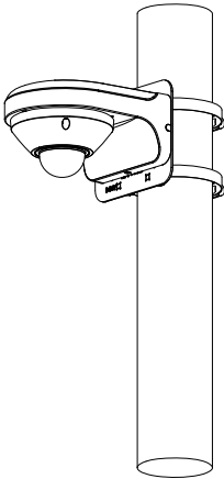
Pole Mount(Vertical)
