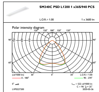
OFPC1_SM340CPSDL12001x365940PCS
