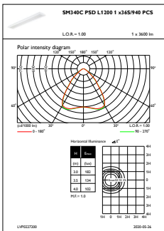
OFPL1_SM340CPSDL12001x365940PCS
