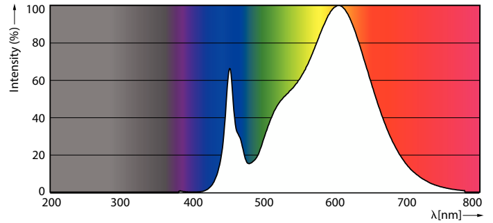
Spectral Power Distribution Colour - MAS LEDtube 1500mm UO 20W 830 T8 SDCM
