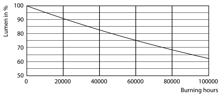
Lumen Maintenance Diagram - MAS LEDtube 1500mm UO 20W 830 T8 SDCM
