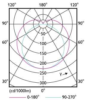
Light Distribution Diagram - MAS LEDtube 1500mm UO 20W 830 T8 SDCM
