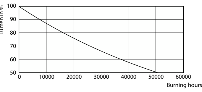
Lumen Maintenance Diagram - MAS LED spot VLE D 5.5-80W GU10 927 36D
