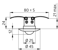
sensor head
