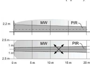
PO-C20 curtain mirror (option)
