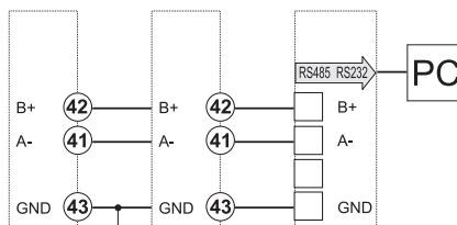
Fig. 28 RS485 port
