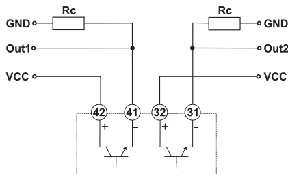
Fig. 25 Static outputs, VCC reference
