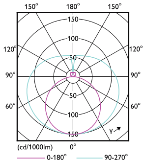
Light Distribution Diagram - CorePro LEDtube 600mm HO 7.7W 3CCT T8
