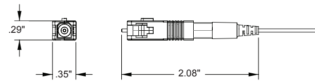
SC Connector
