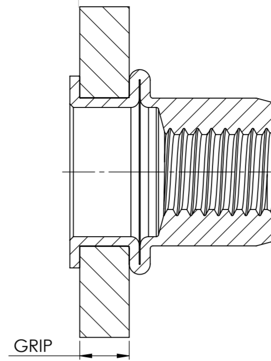
AFTER PLACING
